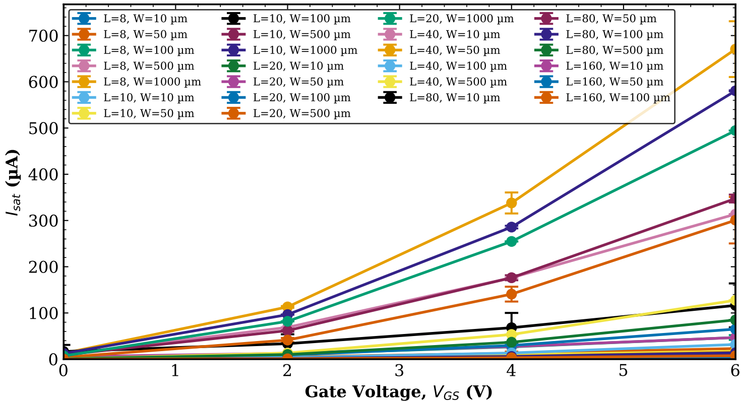
TFT1 Combined (Tr. 1 & 2) Saturation Current vs V_{GS} (mean \pm std)
